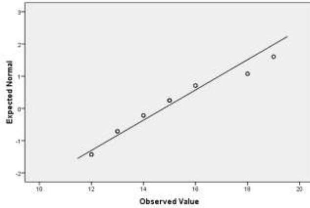
Normal Q-Q Plot of Pretest Total
