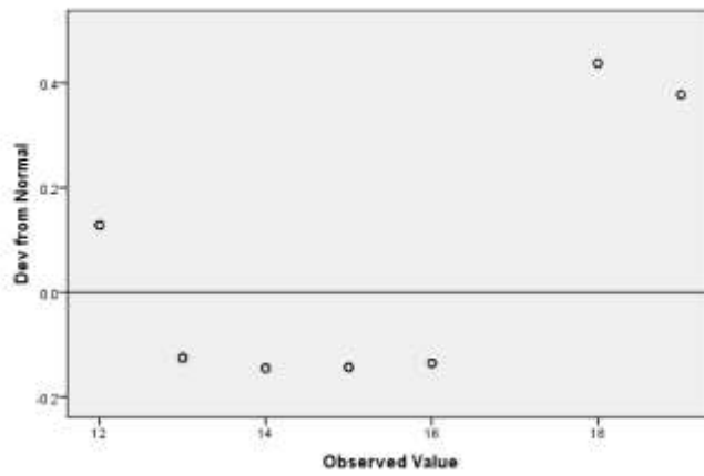
Detrended Normal Q-Q Plot of Pretest Total
