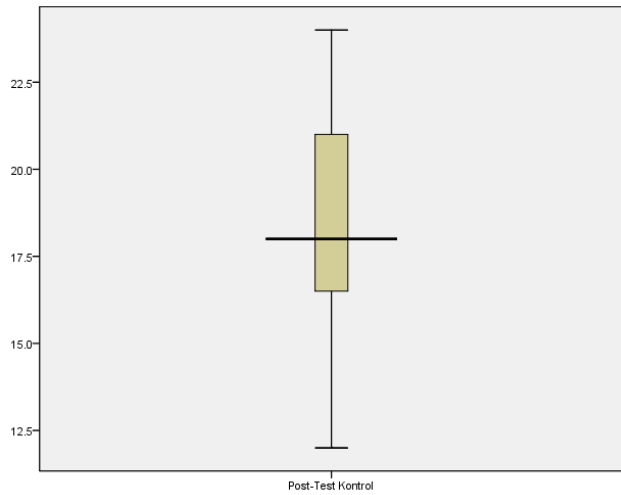
Paired Samples Statistics
