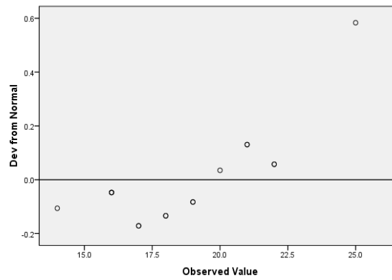
Detrended Normal Q-Q Plot of Pre-Test Eksperimen
