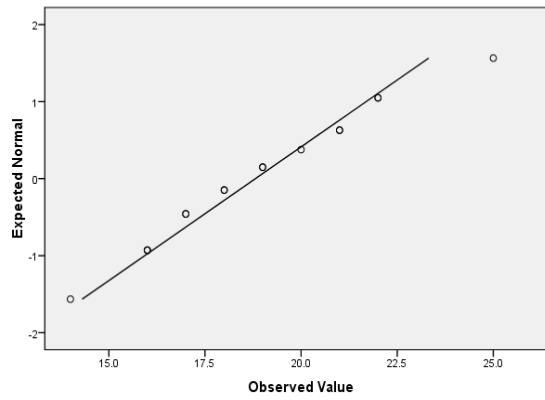
Normal Q-Q Plot of Pre-Test Eksperimen
