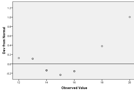
Detrended Normal Q-Q Plot of Post-Test Eksperimen
