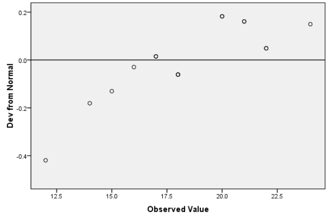
Detrended Normal Q-Q Plot of Post-Test Kontrol
