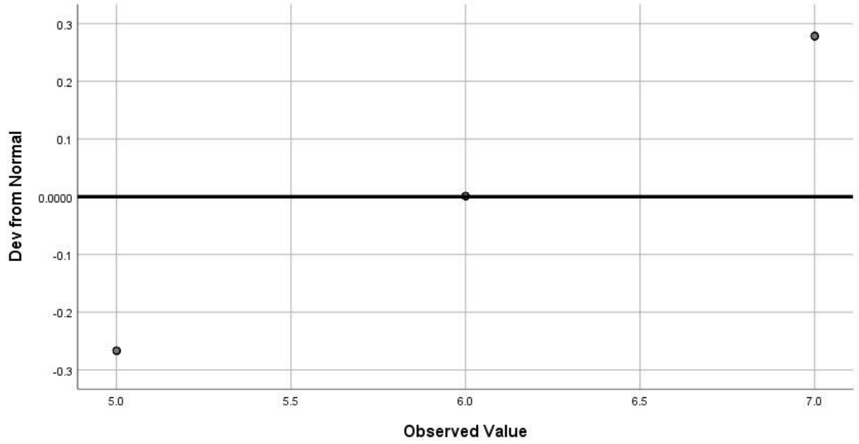
Detrended Normal Q-Q Plot of HASIL for KELAS= 2.00
