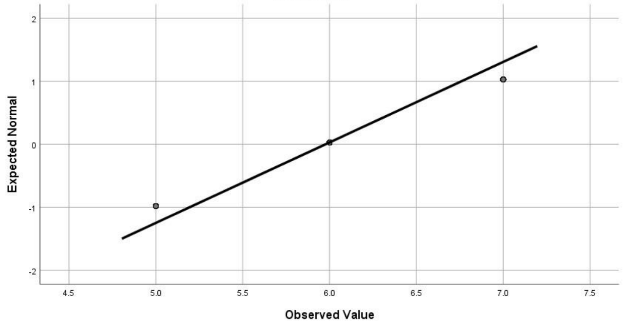
Normal Q-Q Plot of HASIL
