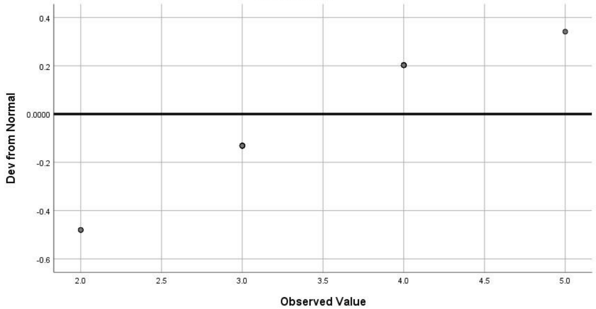
Detrended Normal Q-Q Plot of HASIL for KELAS= 3.00
