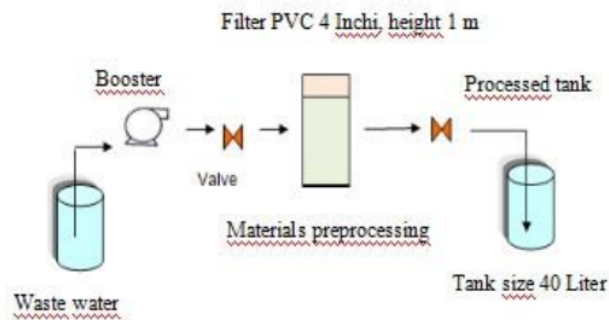
Figure 2. Reactor Design
