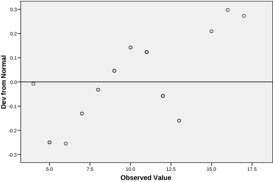
Detrended Normal Q-Q Plot of PRE TEST
