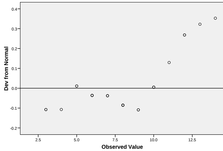
Detrended Normal Q-Q Plot of POST TEST
