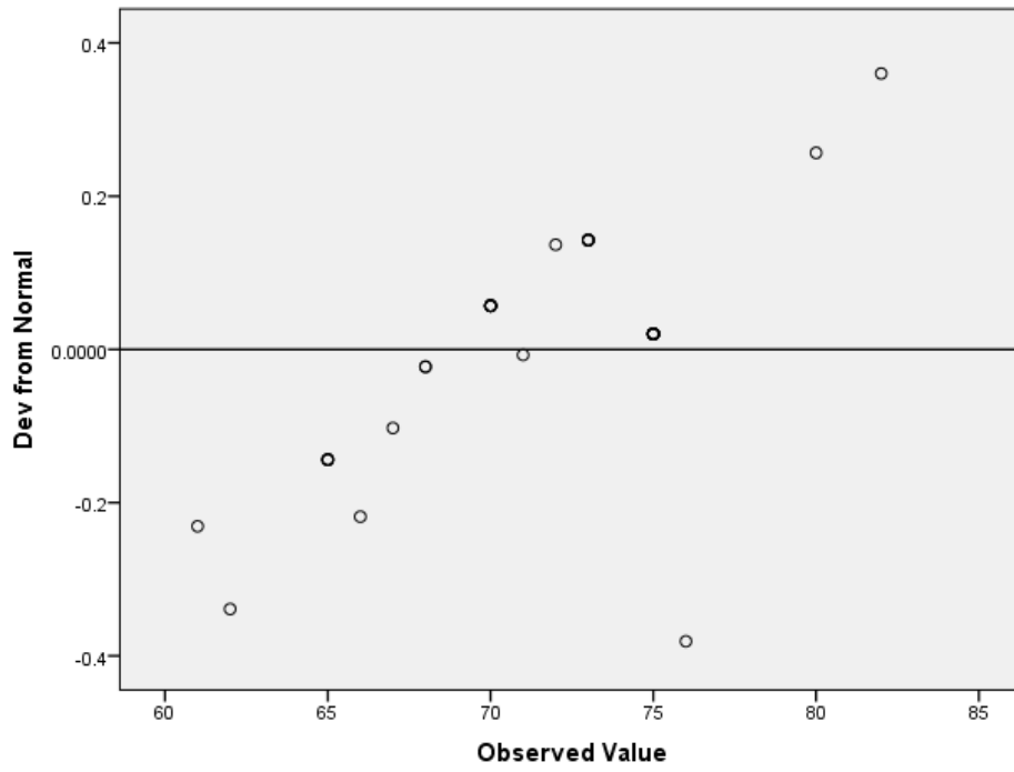
Detrended Normal Q-Q Plot of PRETEST RESPONDEN
