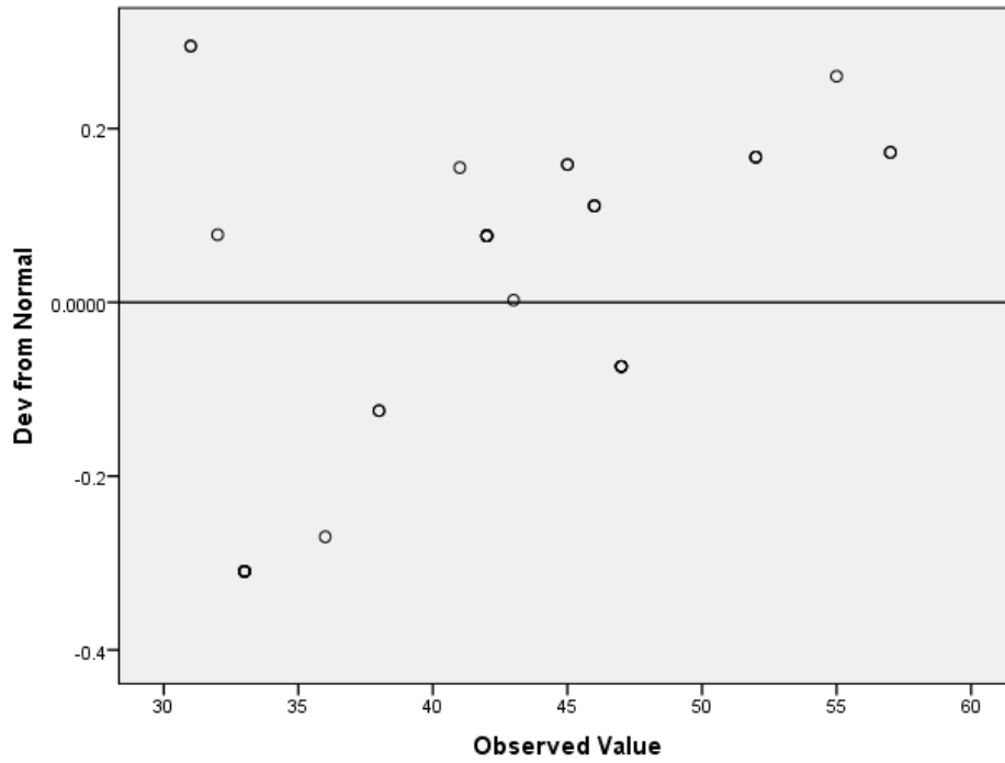
Detrended Normal Q-Q Plot of POST RESPONDEN
