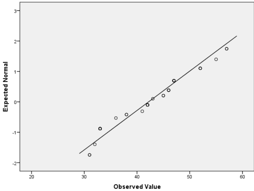
Normal Q-Q Plot of POST RESPONDEN
