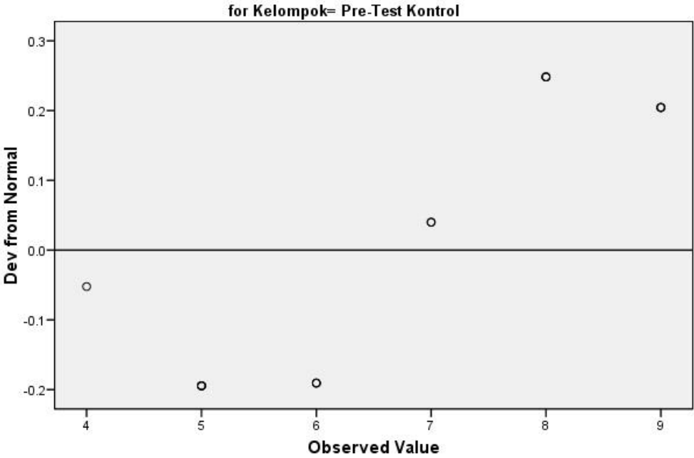
Detrended Normal Q-Q Plot of Skala Nyeri
