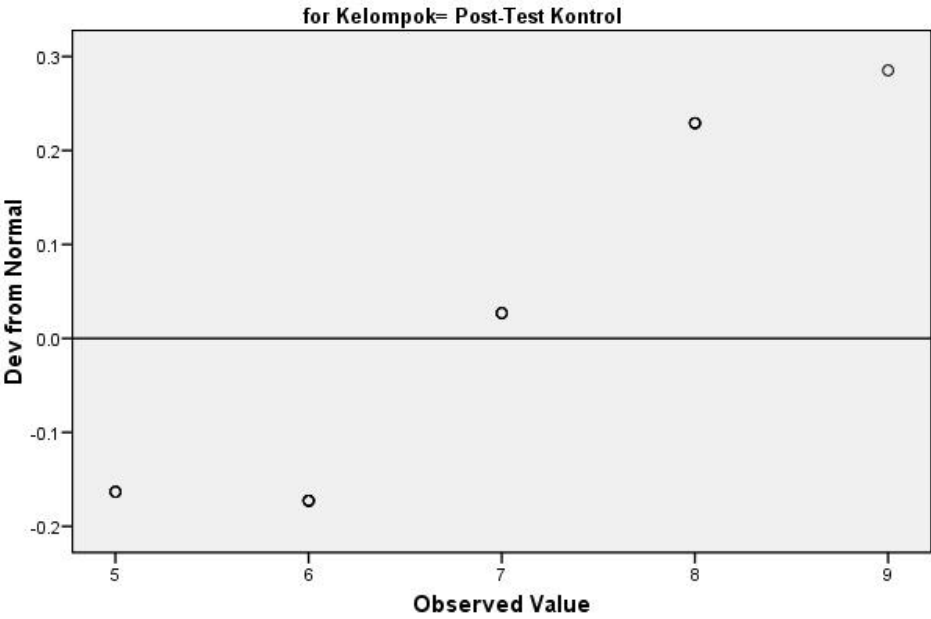
Detrended Normal Q-Q Plot of Skala Nyeri
