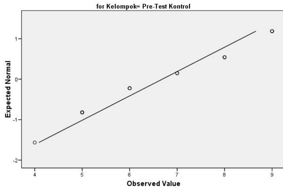
Normal Q-Q Plot of Skala Nyeri
