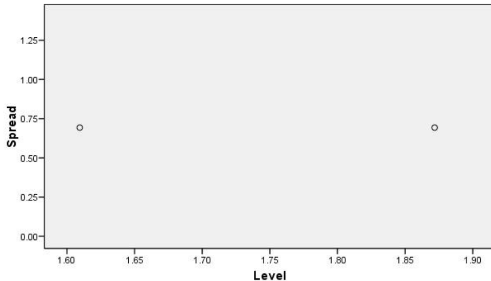
Spread vs. Level Plot of Hasil by Kelompok
