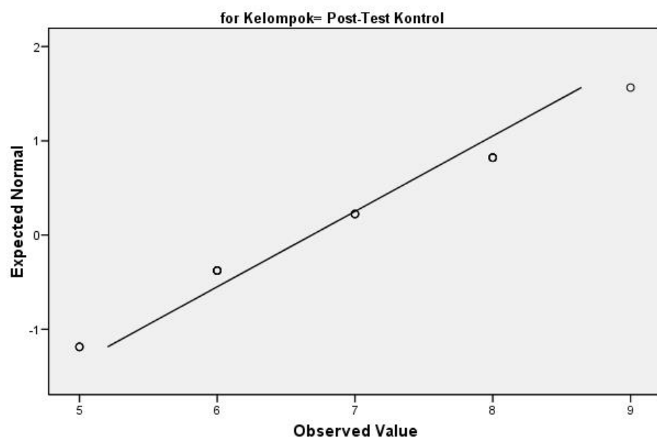
Normal Q-Q Plot of Skala Nyeri
